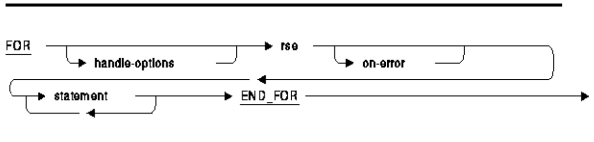
Example 5–3 FOR Format
